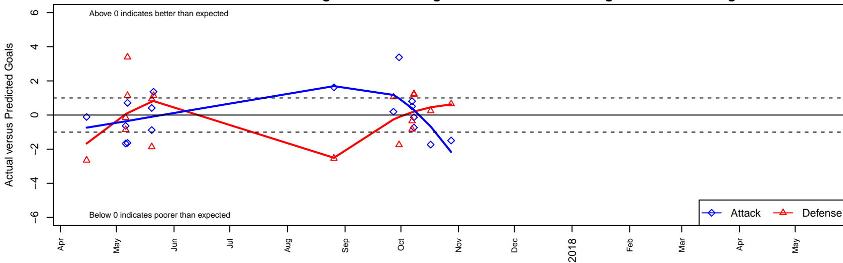
Canyon Optimist Inferno B05 Dots are actual minus expected GF (blue circles) and GA (red triangles). Blue line is smoothed change in attack strength. Red is smoothed change in defense strength.
